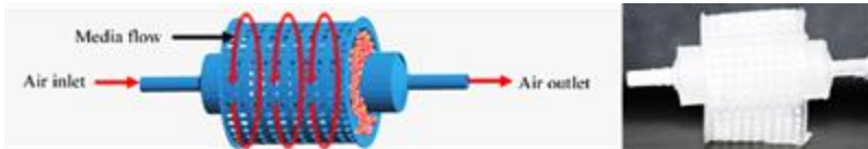
CAD Model and 3D printed structures of next generation miniature bioreactor
