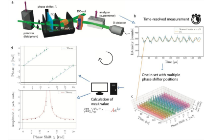
Testing commutation relation (Performed in Atom institute, Vienna)
