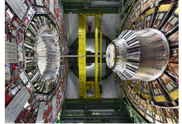
The CMS detector at the LHC
