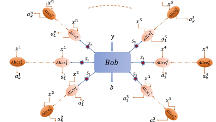
Device-independent nonlocal correlation in Star-network
