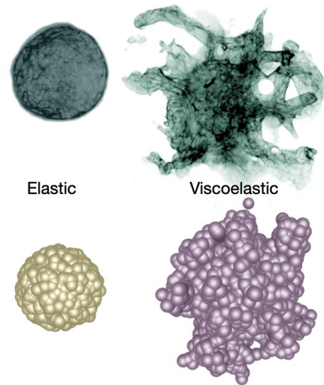
Tissue growth in viscoelastic matrix
