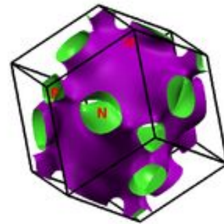
Fermi Surface of LaRu_4P_{12}
