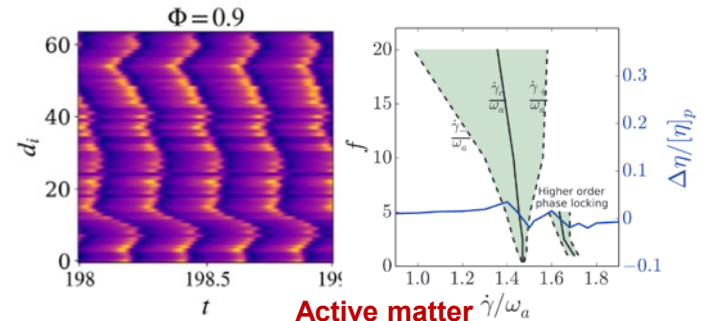
Active matter \dot{\gamma}/\omega_a
