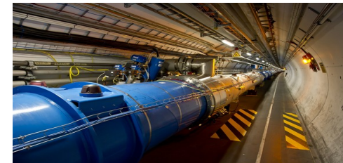
The Large Hadron Collider
