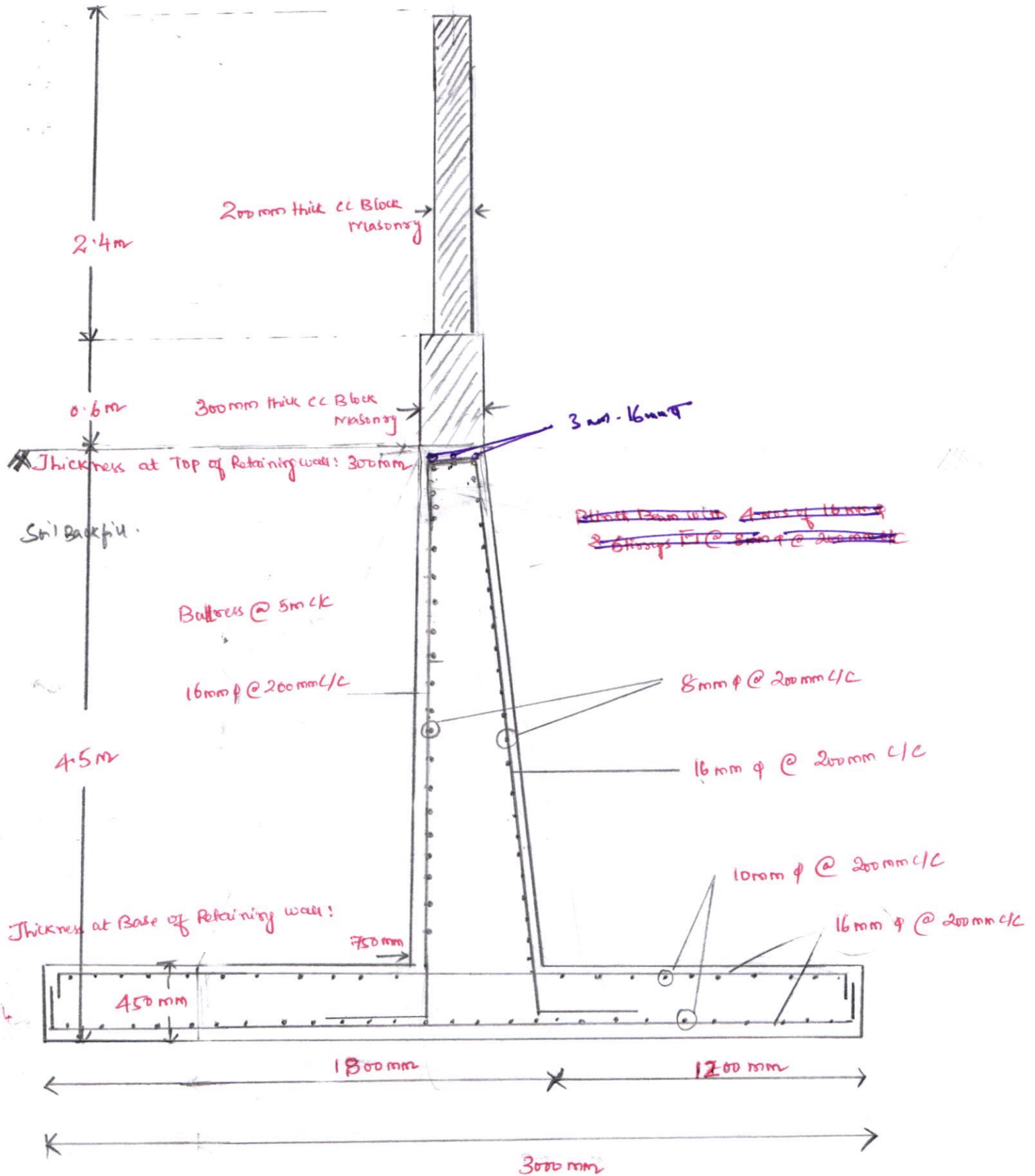
TYPICAL CROSSSECTION DETAILS
