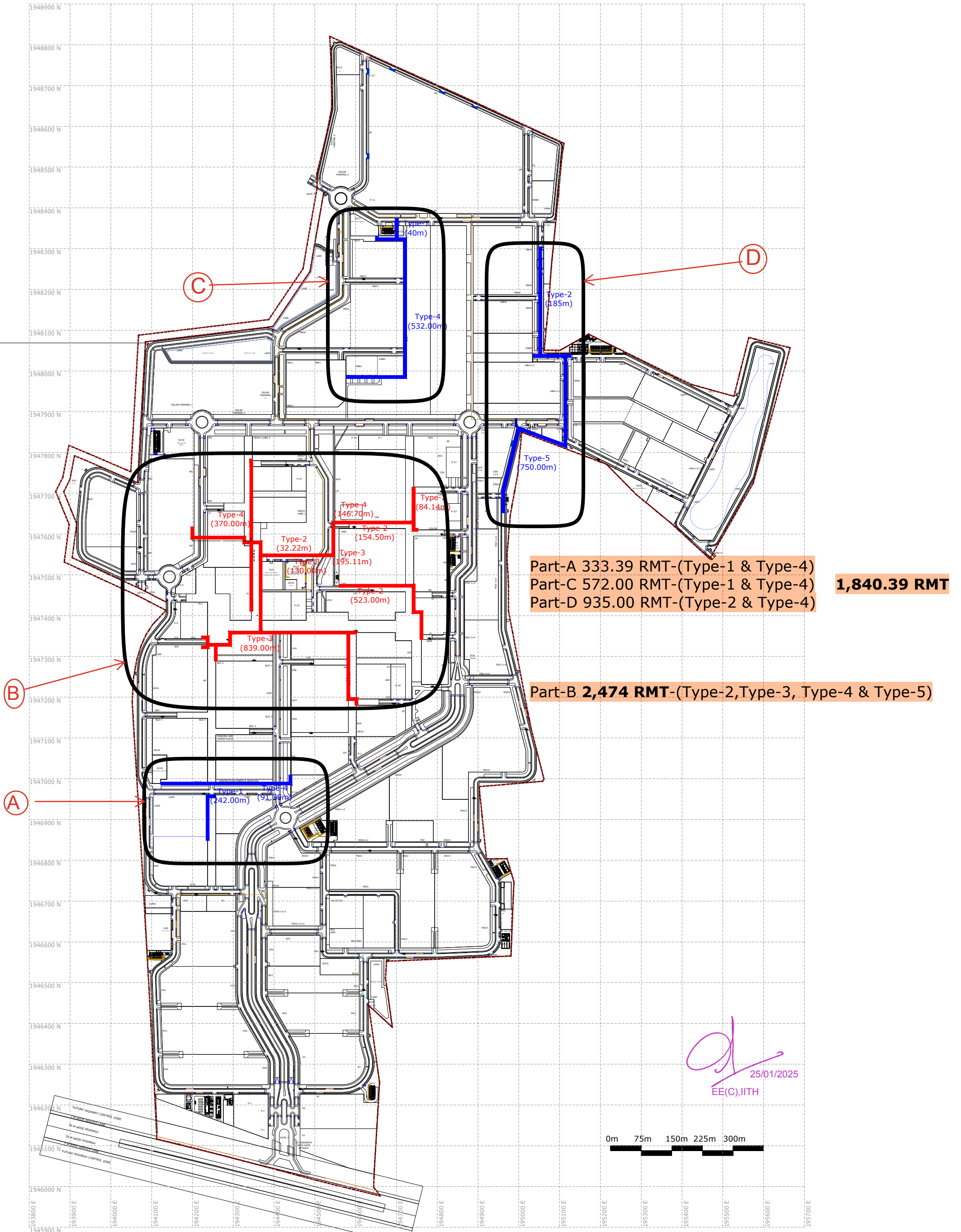
Proposed civil water proofing works inside of infra- related electrical and HVAC trenches of works at IIT Hyderabad, Kandi, Sangareddy.
