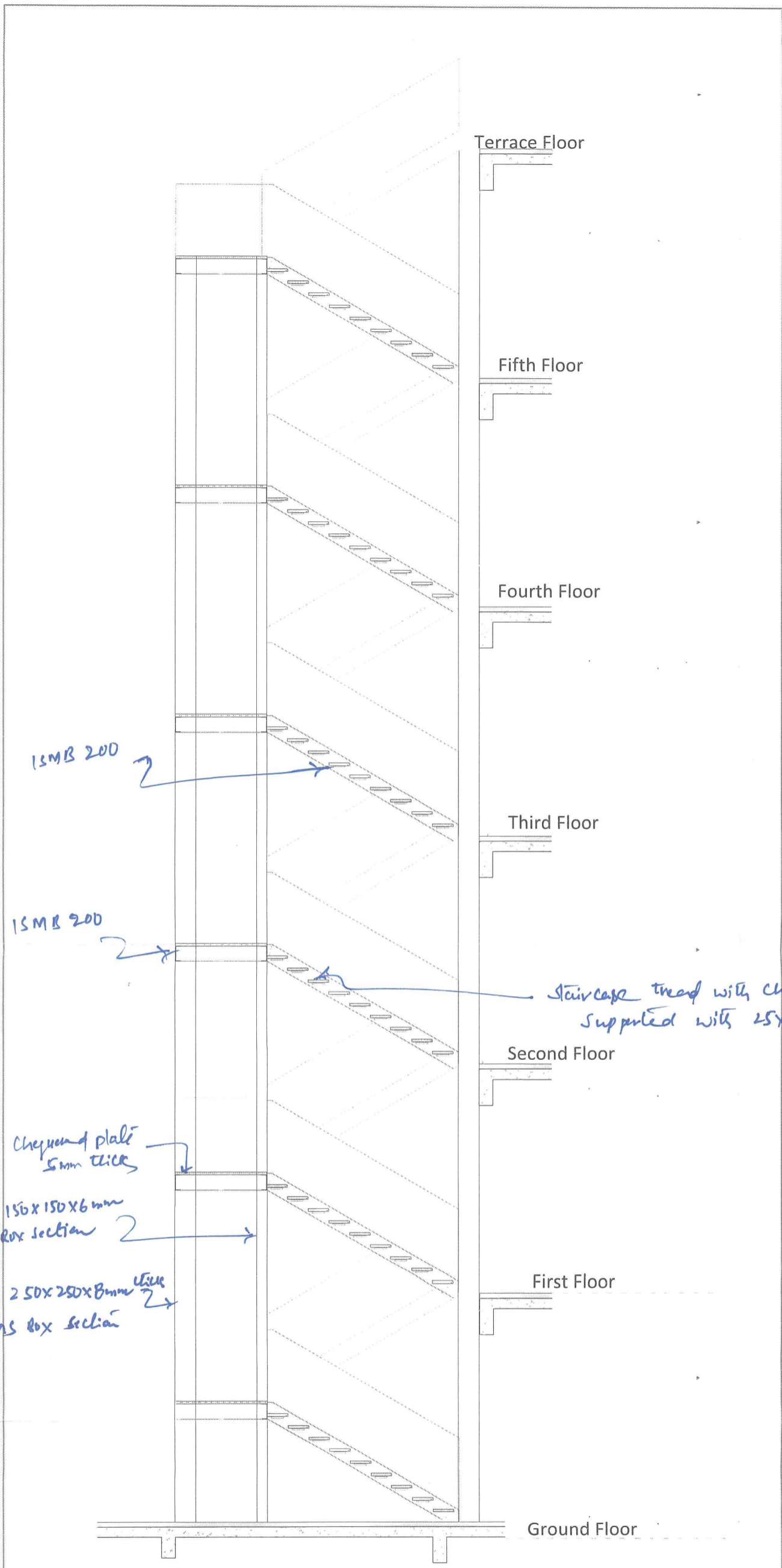
Staircase Detail Section
