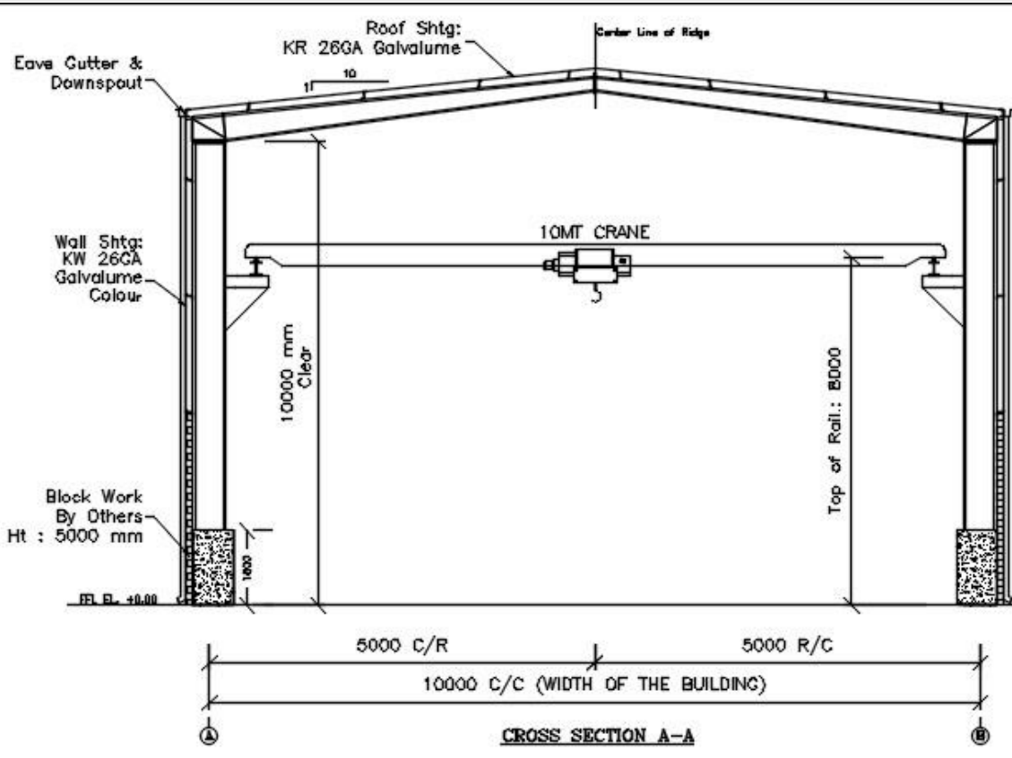
Figure 2. Cross section elevation
