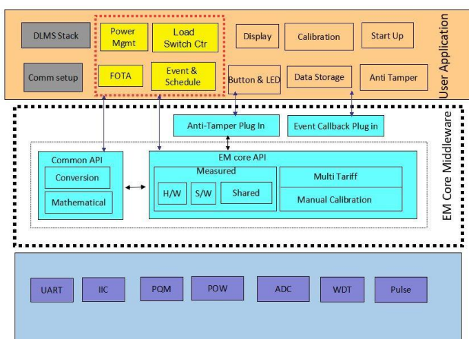
Figure-1: Components of the Smart meter
